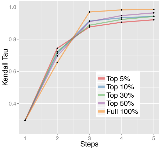
Figure 3: Growing Rings using only the nodes with highest PageRank. The plot shows the average values of the Kendall- \tau at each step computed for all the subgraphs.
