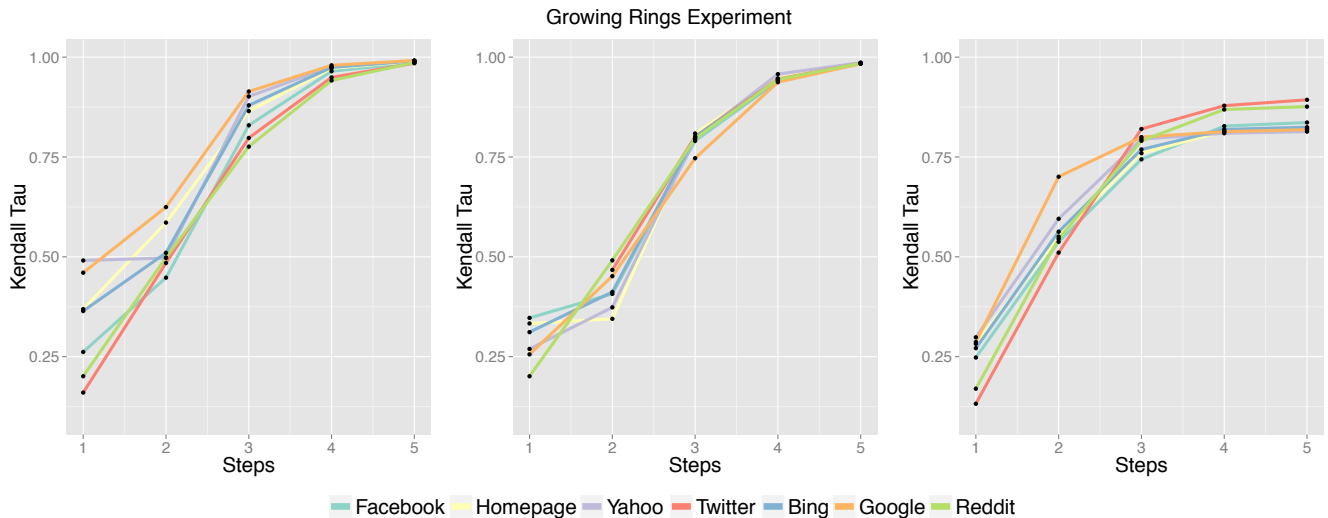
Figure 2: Growing Rings experiment on: (left) original subgraphs built based on the referrer URL, (center) seven subsubgraphs with very similar size, (right) seven subgraphs random selected from the full graph, where each of them has the same size of one of the original.
